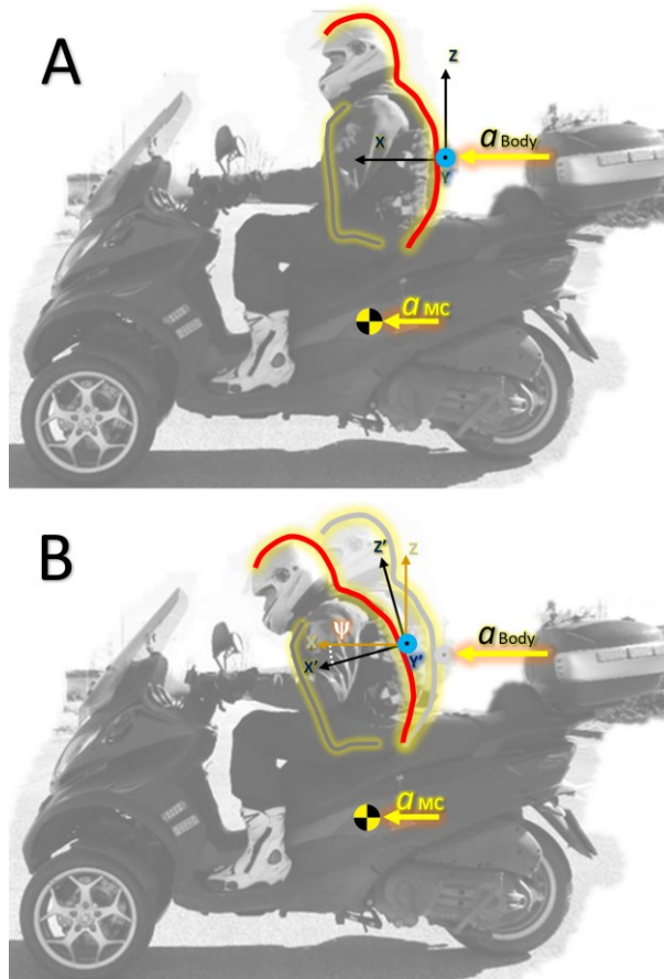
9 Figure 2– Example of vector of longitudinal acceleration of the motorcycle ( a_{MC} ), longitudinal acceleration of upper-body 10 ( a_{Body} ), and differences in pitch ( \psi ) for upper-body. A) trunk at right angle; B) flexion movement of \psi radians. Pitch-rate 11 > 0 refers to forward pitch rotation (flexion) and a_{Body} < 0 to backward acceleration
